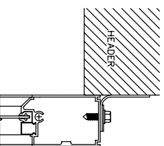
HEADER SEAL
