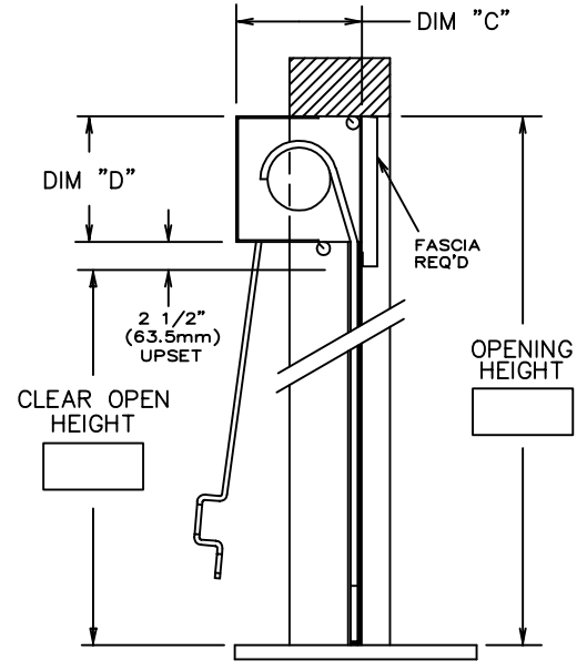
"SECTION THRU-OPENING"
