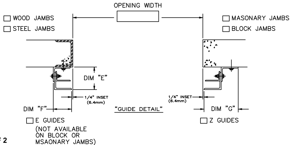
"SECTION THRU-OPENING"
