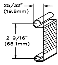
SLAT MODEL "FP"
